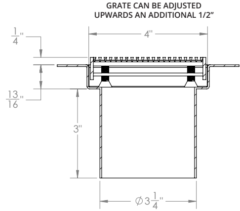
SECTION 1-1
