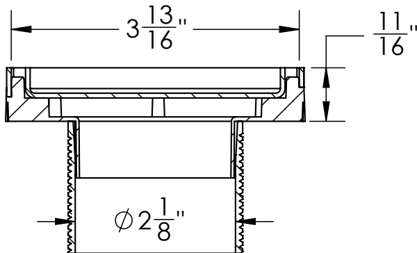
SECTION 1-1
