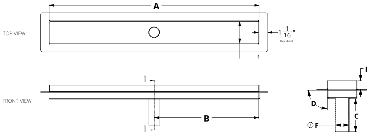
SECTION 1-1
