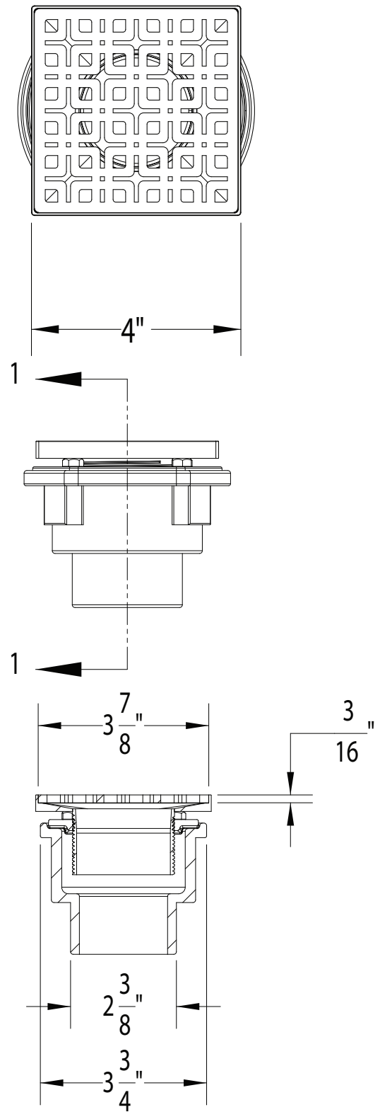
SECTION 1-1
